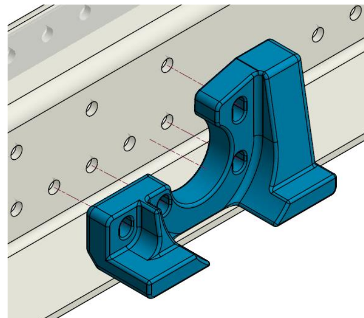
AE080112 CENTER LOCK RIGHT
