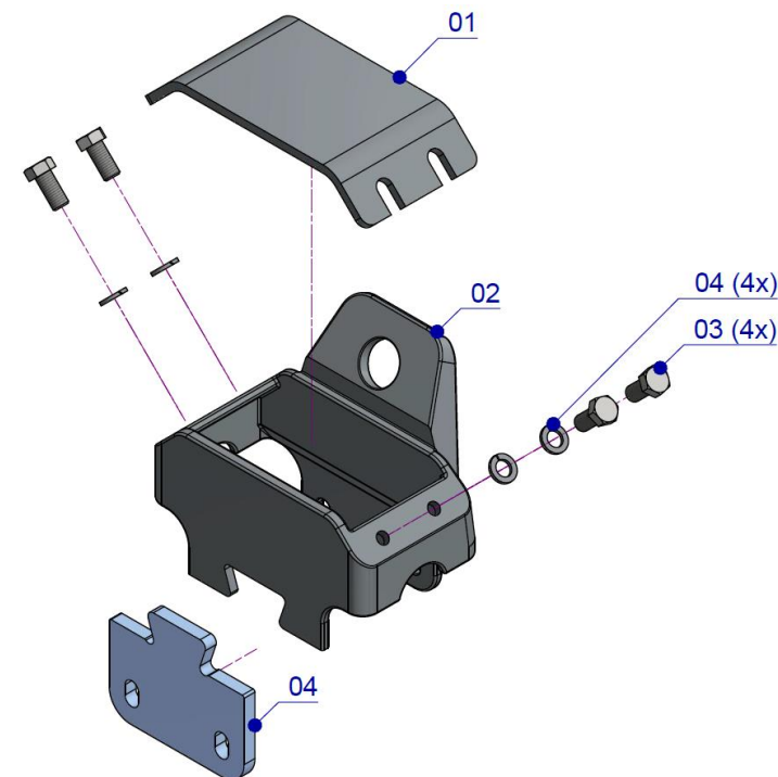
AE090094 (AE080070 only for 26T-49/51/53 systems)
